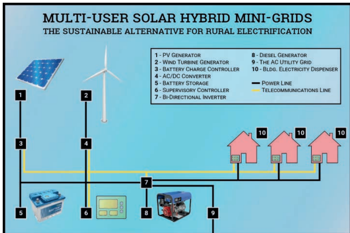
Figure 1: Sample of a renewable mini-grid with DC distribution
