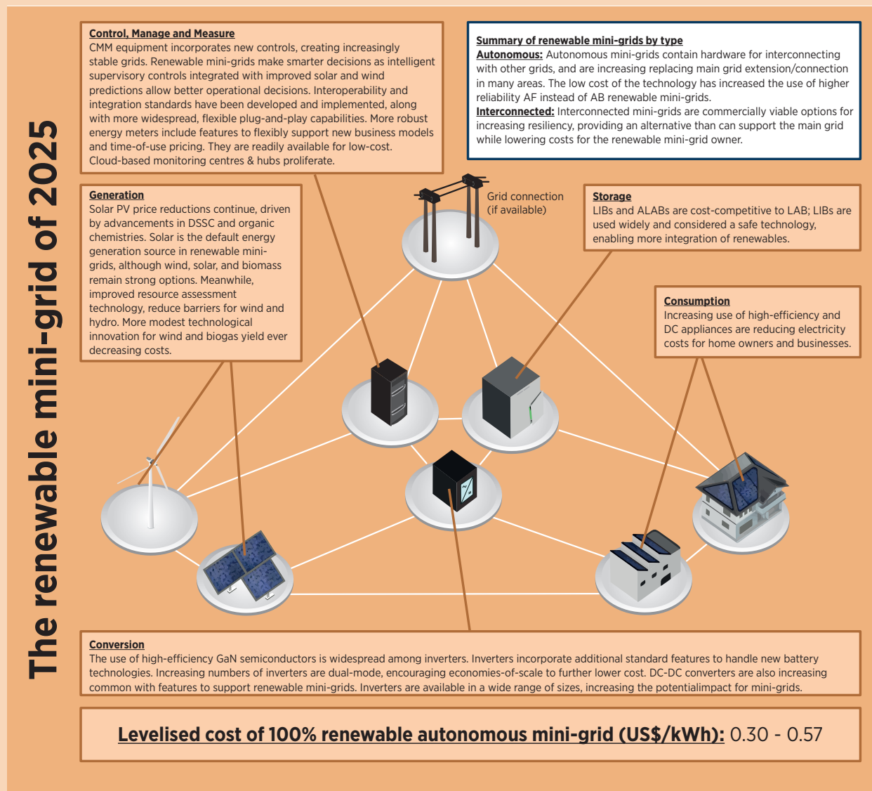
Figure 20: The renewable mini-grid of 2025
