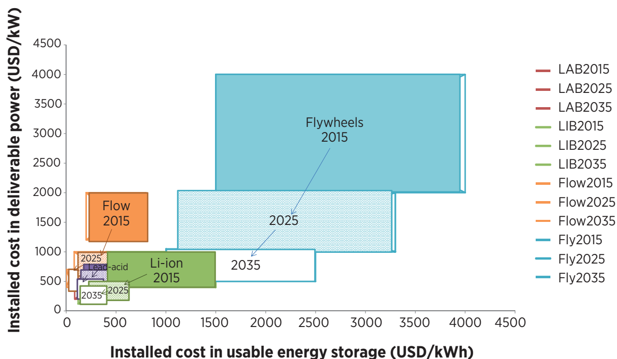
Figure 12: Storage technology cost ranges in 2015, 2025 and 2035 depicted in USD/kW vs. USD/kWh
