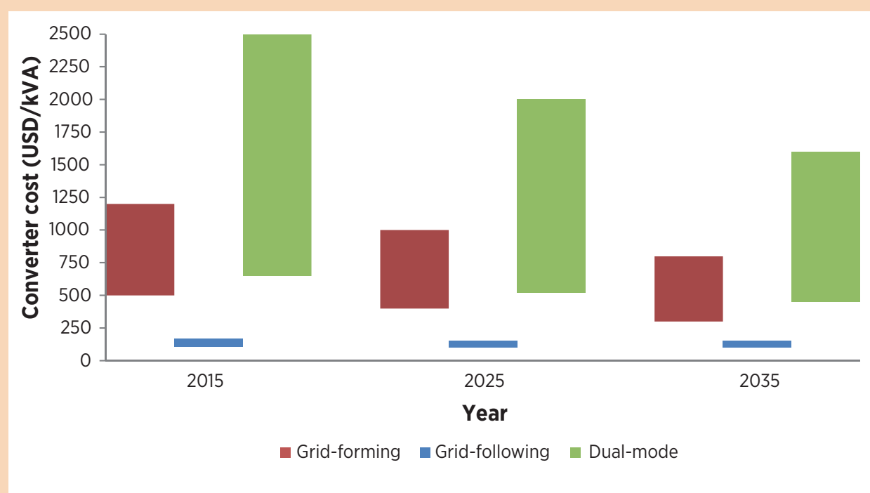
Figure 16: Converter technology cost ranges in 2015, 2025 and 2035
