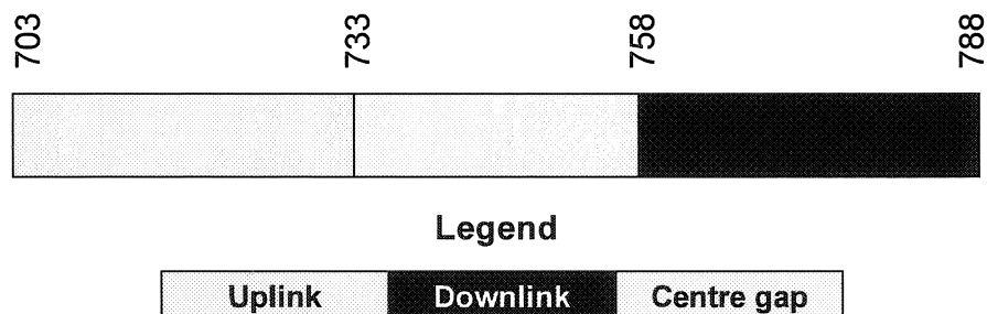
Figure 4: Channel arrangements for IMT700
