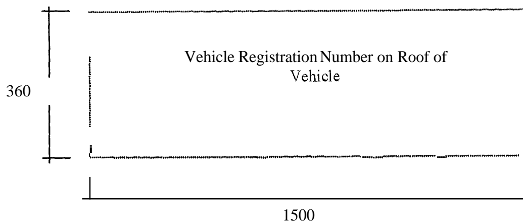
Figure 5 – Design Specification of the Marker on the roof of the Vehicle
